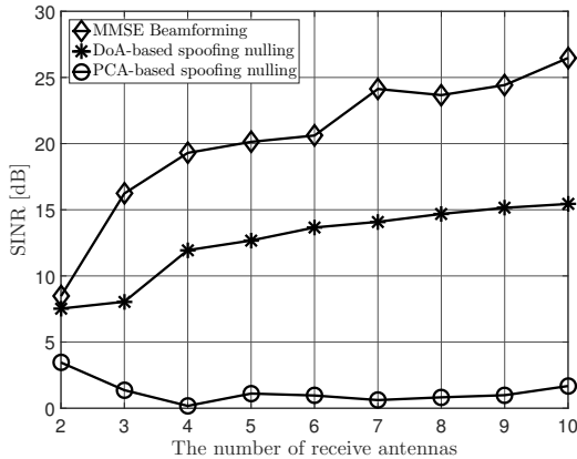
Fig. 5. SINR performance of the proposed MMSE beamforming-based spoofing mitigation technique
