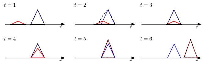
Fig. 2. GNSS Spoofing attack process in sophisticated spoofing scenario [7].
