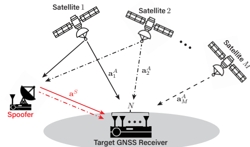
Fig. 1. System model where a single spoofer with a single antenna and a target GNSS receiver with an array antenna exist at a fixed position.
